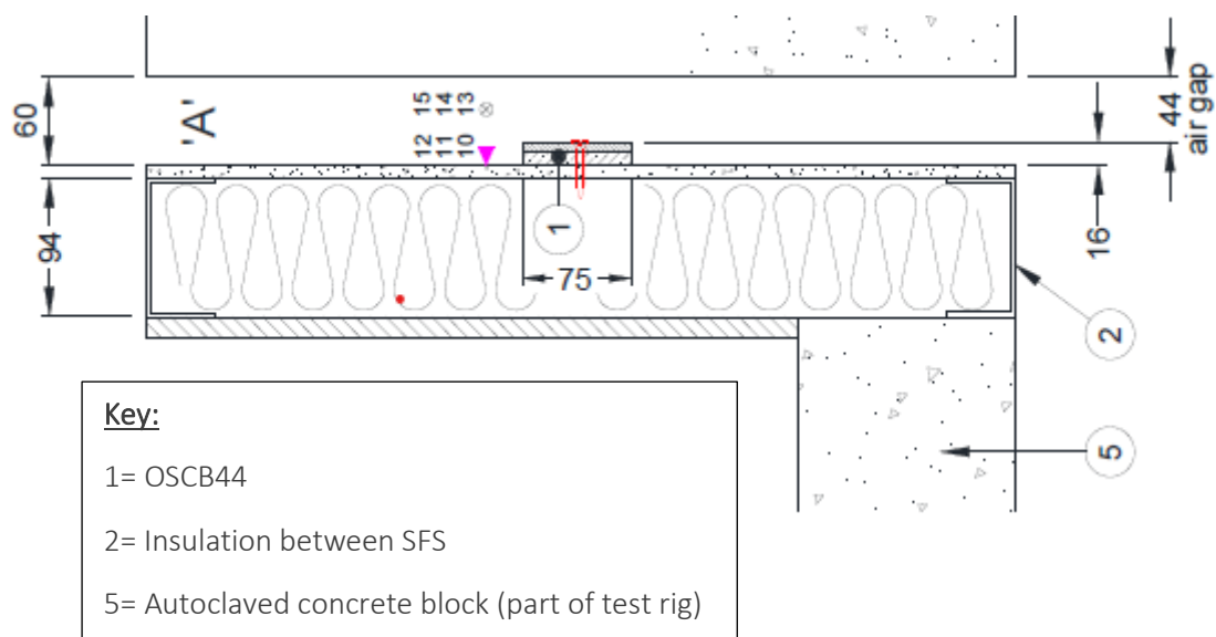
Figure 1 – Typical Installation of OSCB44 Cavity Barrier without inner wall insulation (Drawing Taken from Warringtonfire report WF 434726)
