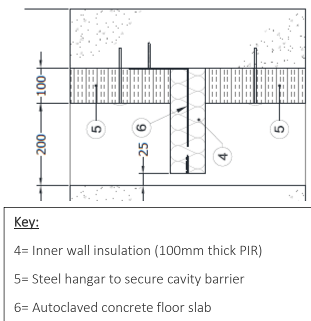
Figure 2 – Typical installation of OSCB44 Cavity Barrier with inner wall insulation (Drawing taken from Warringtonfire report WF 394958)
