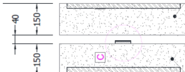
Figure 1 – Typical installation of OSCBPLUS25 (circled) without insulation on the inner wall (Drawing taken from Warringtonfire WF 433220)
