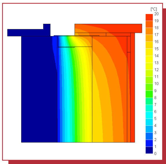
Temperature distribution illustrating heat loss at a window opening where ARC Contract-Closer is fitted.
