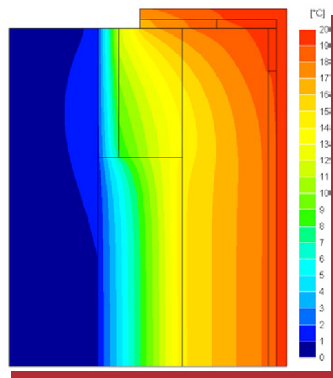
Above: Temperature distribution illustrating heat loss at a window opening where ARC Insulated DPC is fitted.
